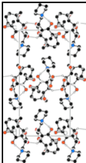
Fig. 2. : Packing view showing the C–H···O and O–H···N hydrogen bonds as dashed lines. H atoms not involved in hydrogen bonding have been omitted for clarity.
